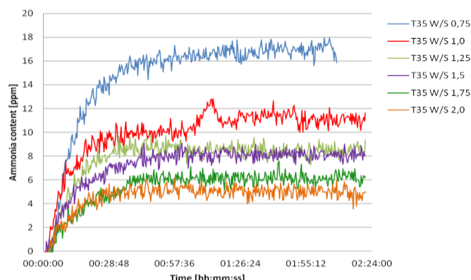
Fig. 3. The concentration level of ammonia discharged from the hydromixture in proportion W/S = 2.0–0.75 in the accepted time of 2.5 hours
